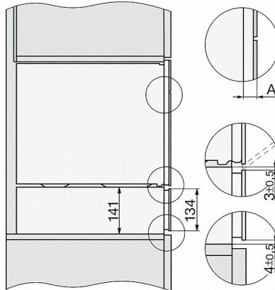
A) 22 mm glass, 23,3 mm stainless steel
