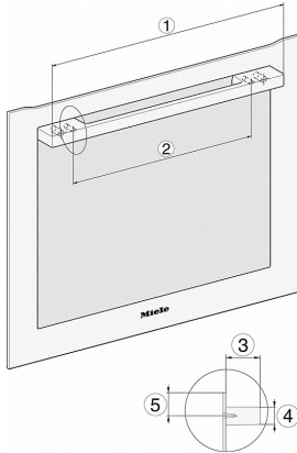
DG2740, DG7140, DGM7340, H2760B/BP, H7140BM, H7x64B/BP, installation drawings
