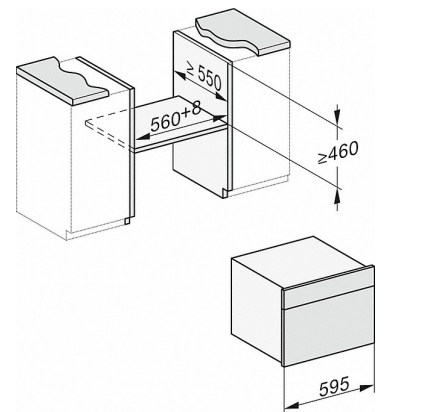
DG7x4x, DGM7x4x, DGC7x4x, DGC7x4xX installation drawings
