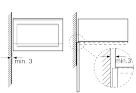
Microwave, corner installation
