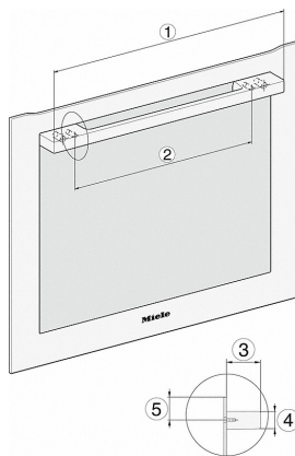
DG2740, DG7140, DGM7340, H2760B/BP, H7140BM, H7x64B/BP, installation drawings
