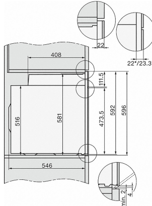
H2x6x-1B/BP/E/EP/I/JP, H2850BP, H7x6xB/BP/BPX, H2x6xB, installation drawings, GB, AUS
