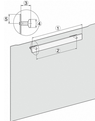
H226x-1B/BP/E/EP/I/JP, installation drawings
