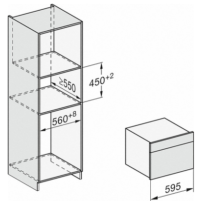
DG7xxx, DGM7xxx, installation drawings
