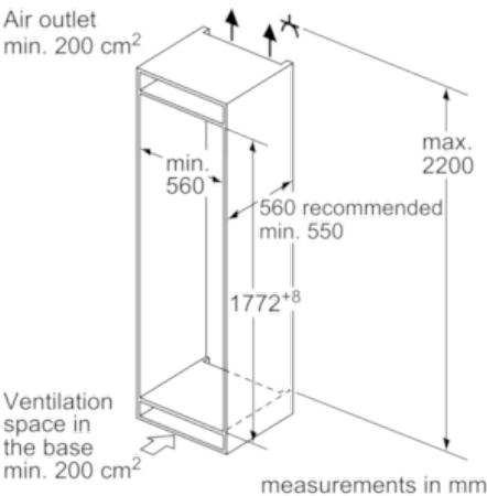
Dimensioned drawings
