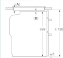
measurements in mm Installation with a hob
