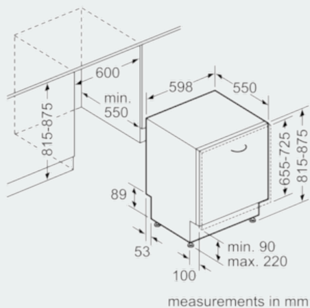
Dimensioned drawings
